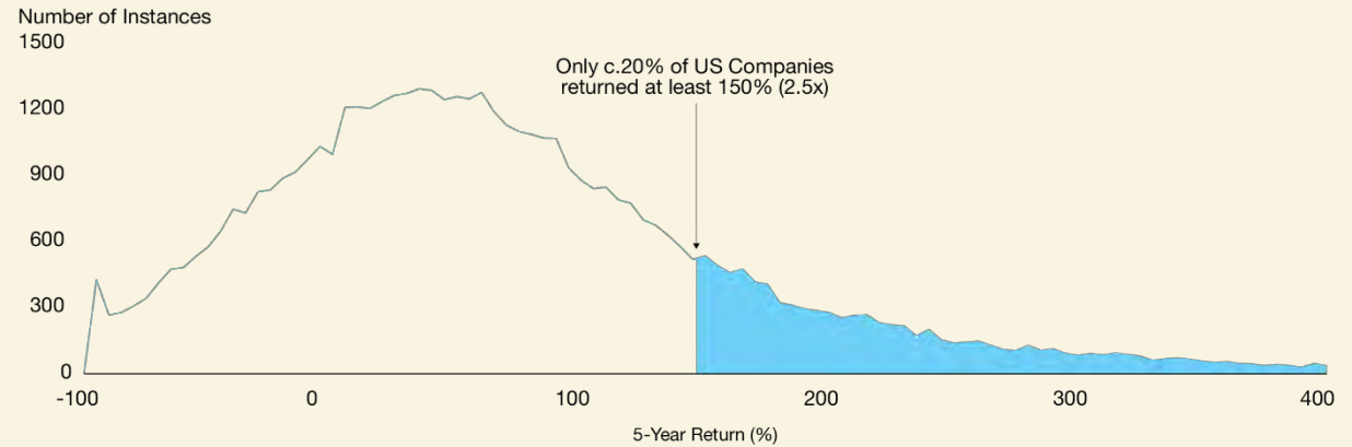
S&P 500 rolling 5 year forward stock returns from 1985-2020
